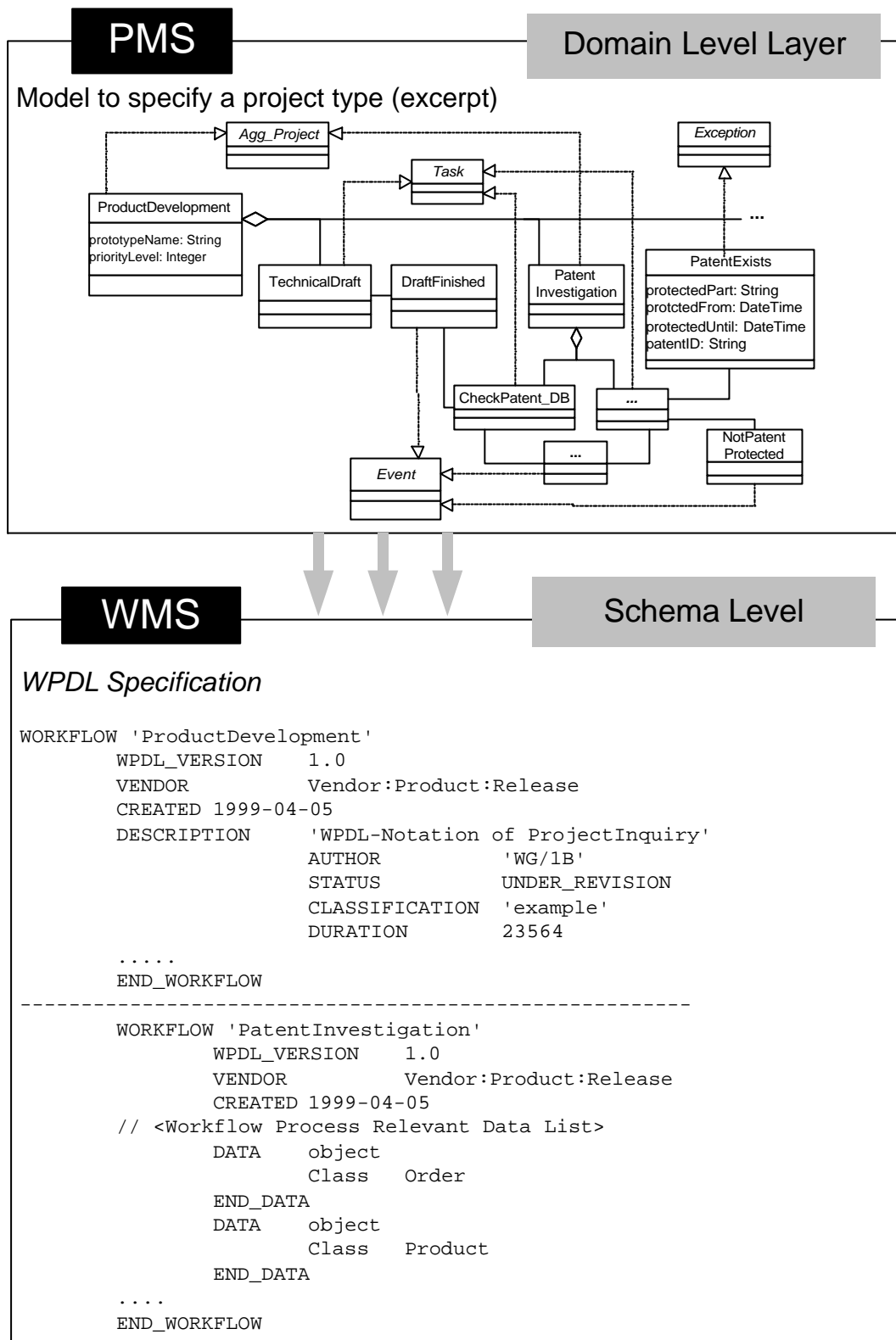
Fig. 3: Object model of a project type and corresponding workflow specification (excerpts)
