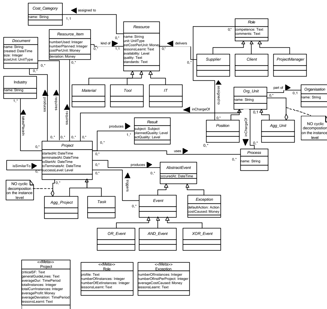
Fig. 2: Excerpt from the object model of the ontology level layer
