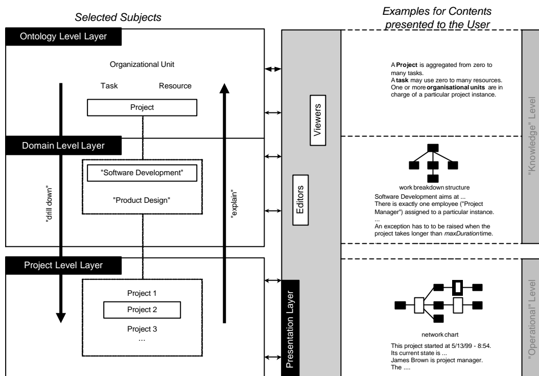
Fig. 1: Overview of the architecture
